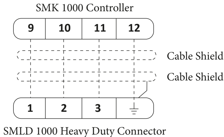
Figure 9: Wiring diagrams
