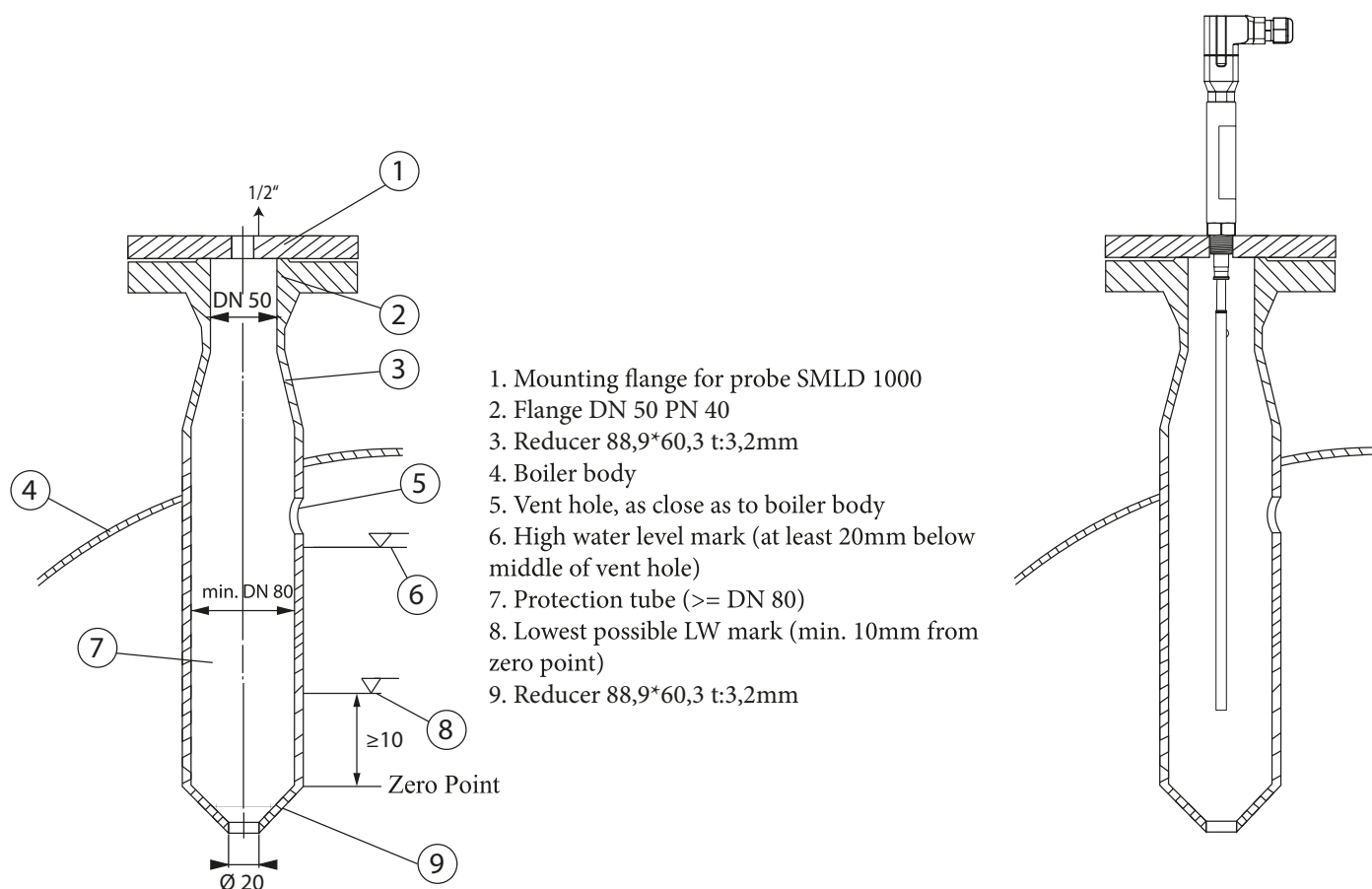
Figure 4: Installation example 1, usage with protection tube inside the boiler.
