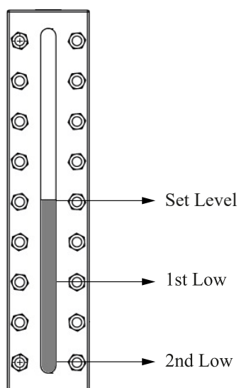
Figure 3 : Low Alarm Levels.
