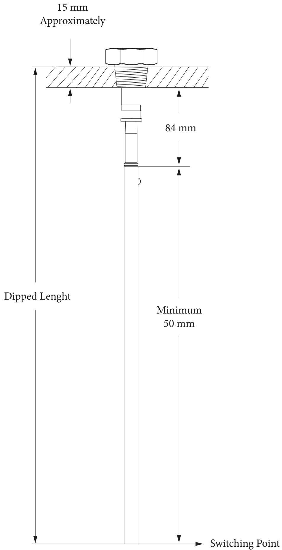
Figure 7 : SMLD 1000 Probe length indication.
