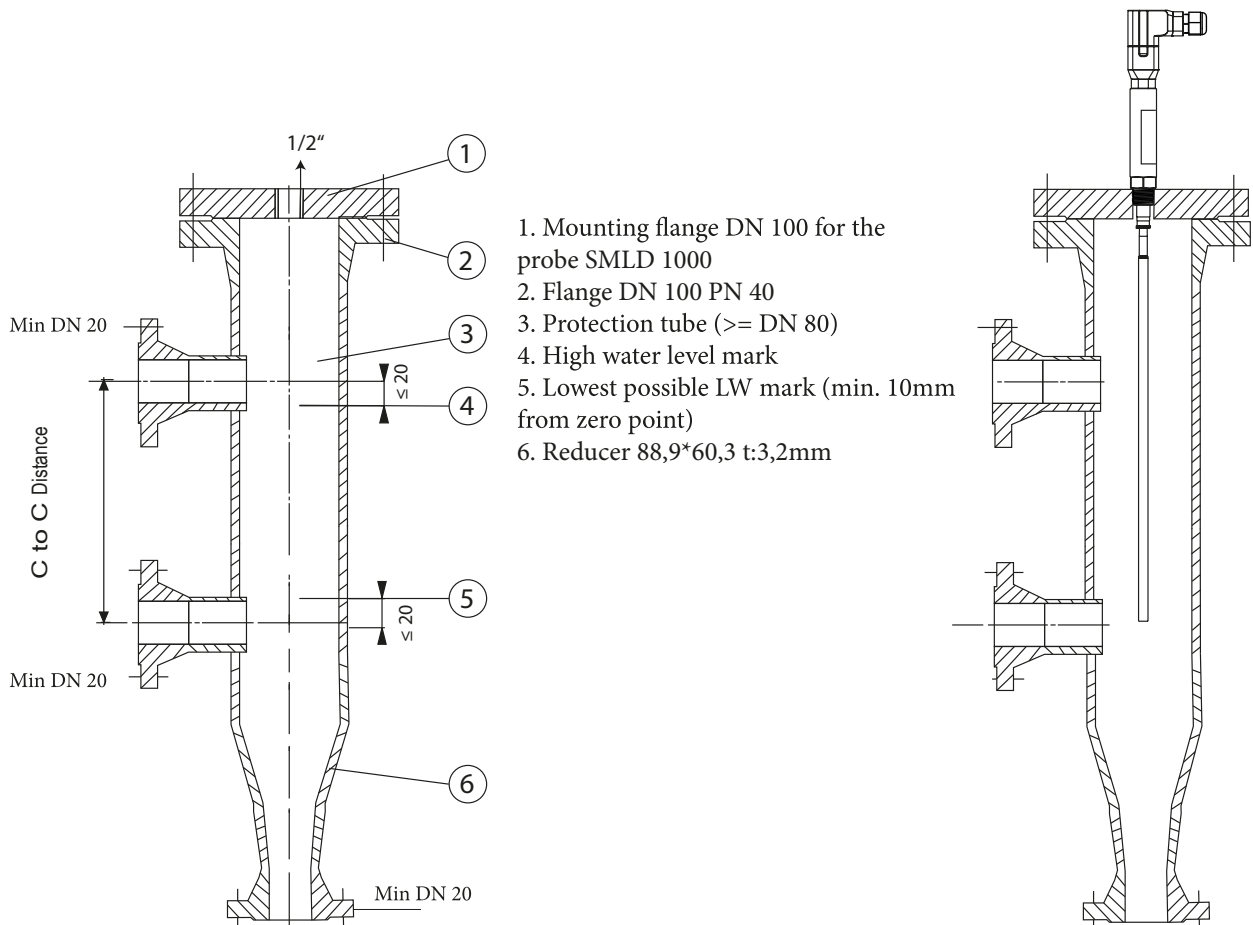
Figure 6 : Installation example 3, usage with protection tube outside the boiler.
